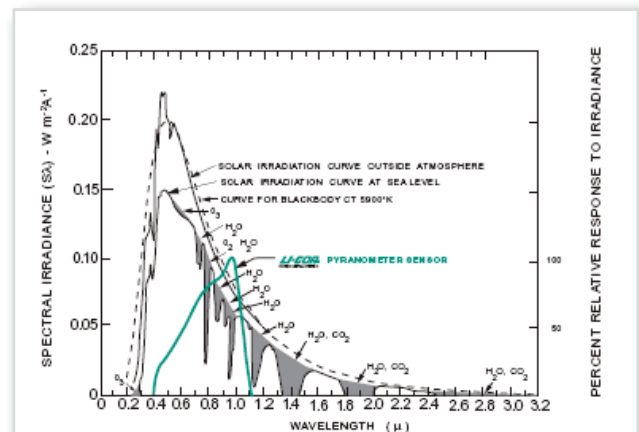
Figure 1. The LI-200SA Pyranometer spectral response is illustrated along with the energy distribution in the solar spectrum (3)
